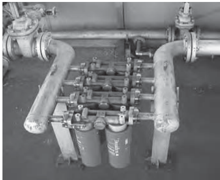
Single-pass Bulk Fuel Filtration System
